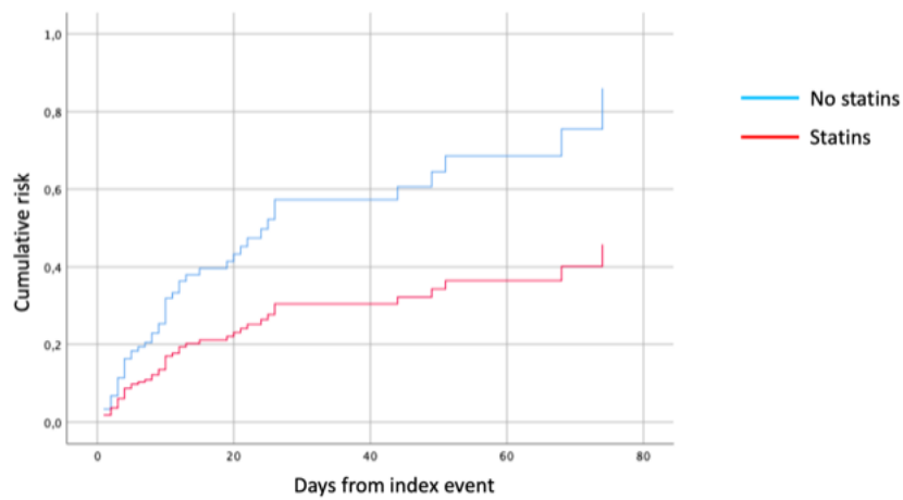
Figure 2: Cox Regression: Statins as an Independent Predictor for Symptomatic Intracranial Hemorrhage.
