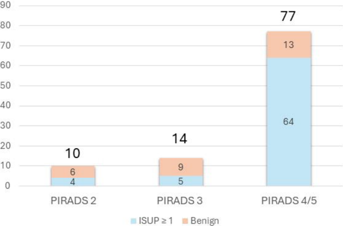
Prostate Cancer proportion per PI-RADS group
