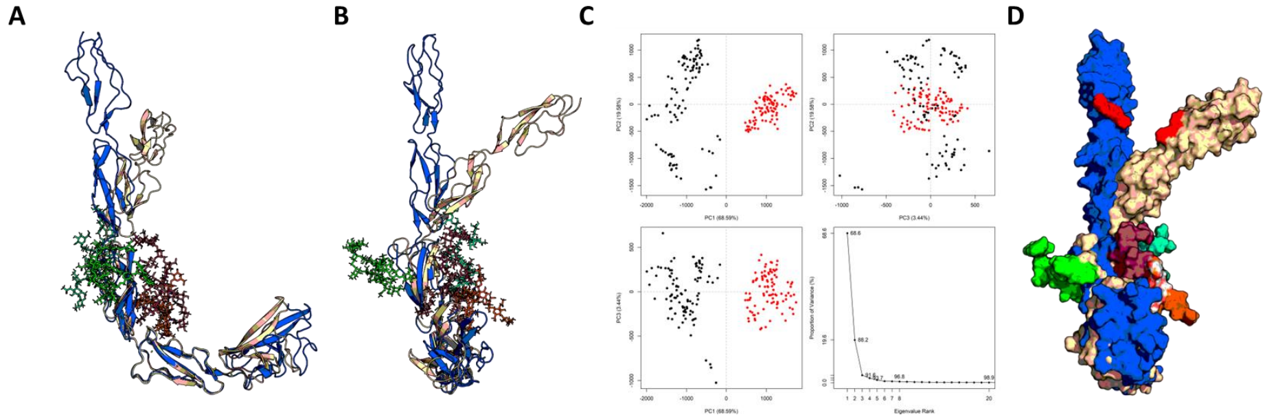
Figure 7: Alignment of the best fitting structures from the molecular dynamics simulations by domain IV (which shows the least difference) highlights the alterations in the orientation of DI and DII (A & B). When combining the top 100 frames of each of the clipped and non clipped B2GPI and conducting a PCA analysis, it shows that the two sets of structures are significantly different with PC1 accounting for almost 70% of differences whilst PC2 accounts for another 19% (C) with the black dots being plasmin clipped and the red dots non-clipped B2GPI, also showcasing the high variability in structures in the plasmin clipped compared to the non-clipped B2GPI. Finally two space models of the best fits are overlaid with the R39-G43 epitope highlights, as can be seen it not simply a case of the protein bending but in the plasmin clipped B2GPI it also rotates exposing the epitope differently, perhaps explaining the increased binding of antibodies in serum to the plasmin clipped B2GPI.
