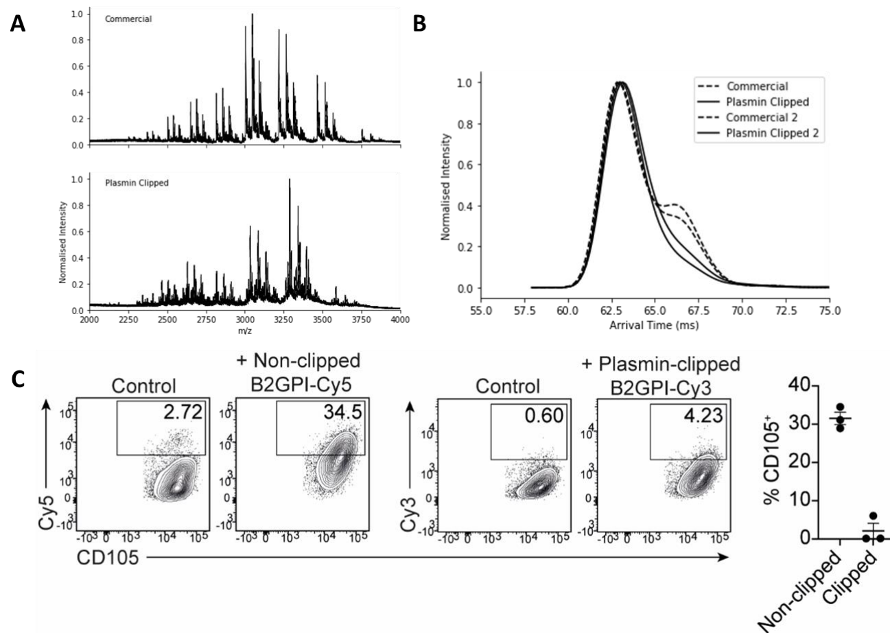
Figure 3: Ion Mobility Mass Spectrometry and FACS analysis. Panel A shows the spectra of both the non-clipped B2GPI (top) and the plasmin clipped B2GPI (bottom), as can be seen both retain a number of glycoisoforms, however, the distribution of charge states is different in the Plasmin Clipped B2GPI suggesting a difference and a more compact conformation. Further to this in B, Ion Mobility data shows in non-clipped B2GPI that there two conformational families, with the dominant conformer corresponding to the earlier peak. In contrast plasmin clipped B2GPI shows a single dominant conformational family, suggesting that cleavage results in the loss of the extended form. Plasmin Clipped B2GPI is known to lose its ability to bind to cell surfaces, as such we conducted FACS with fluorescently labelled B2GPI (clipped and non-clipped) on HUVEC cells. As can be seen, non-clipped B2GPI (Cy5 labelled) bound to approximately 3-35% of cells (2ug B2GPI, 500,000 cells) whilst plasmin clipped B2GPI bound between 0 and 4.5% of cells, significantly less.
