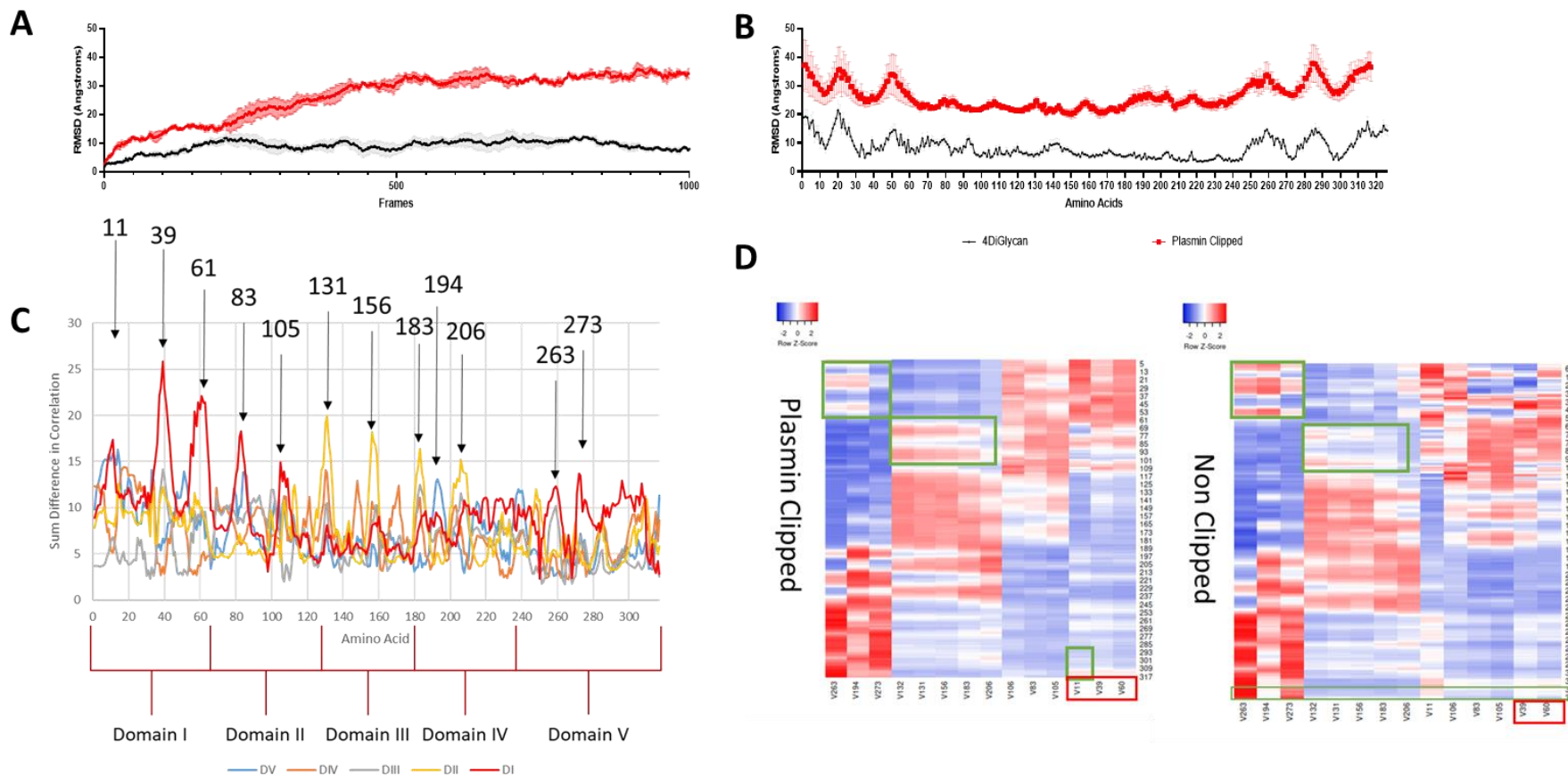
Figure 8: Molecular simulation of B2GPI. Panel A and B show the RMSD of non-clipped B2GPI across the simulation compared to plasmin clipped B2GPI (A) and the same comparison by amino acid (B). As can be seen in both measures plasmin clipped B2GPI has a far greater flexibility and movement suggesting a significant structural change occurs during cleavage. This corroborates the wet lab work suggesting a different structure and higher variation in structure. Further to this an analysis of intra-protein networking showed that significant differences were seen across multiple domains in the DCCM matrixes, this is demonstrated in (C) where sum differences in correlation per amino acid vs domains are plotted. As can be seen the red line (DI) shows the most significant changes in movement correlations with both itself and long range to DV, similar the yellow line (DII) shows significant alterations in correlation with the 3 rd (DIII) and 4 th (DIV) domain. A number of amino acids are picked out as high points for variation, pointing to a pathway throughout the protein effected by the modification. Plotting these variations on a heatmap for their correlation with other domains and themselves (D) reveals a backbone of amino acids which correlate with domains throughout the protein. Interestingly, significant alterations are seen in how these amino acids signal together, the green boxes show areas where correlations are altered, with more correlation between V132-V206 with DII in the Plasmin Clipped, whereas these are less strongly
