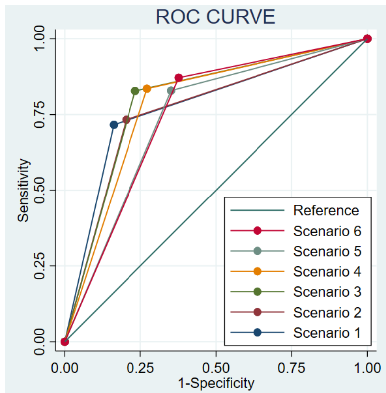
Figure 2. ROC curve for 6 scenarios using the classical method as a classifier.
