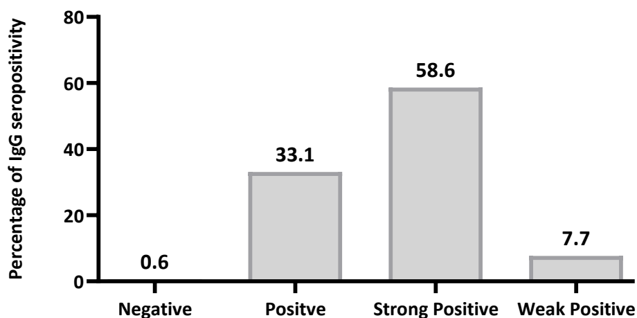
Figure 2: Seroprevalence of SARS-CoV-2 IgG antibody concentrations among non-vaccinated participants (N=169)
