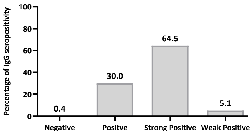
Figure 1: Seroprevalence of SARS-CoV-2 IgG antibody concentrations among the study participants (N=273)
