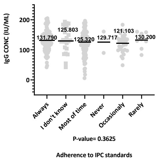
M] IgG concentration by adherence to IPC
