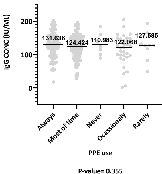
M] IgG concentration by adherence to IPC
