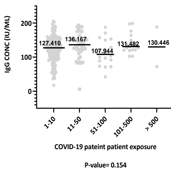
N] IgG concentration by COVID-19 patient exposure
