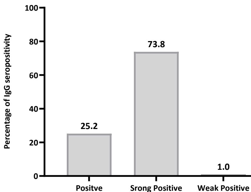
Figure 3: Seroprevalence of SARS-CoV-2 IgG antibody concentrations among vaccinated participants (N=103)
