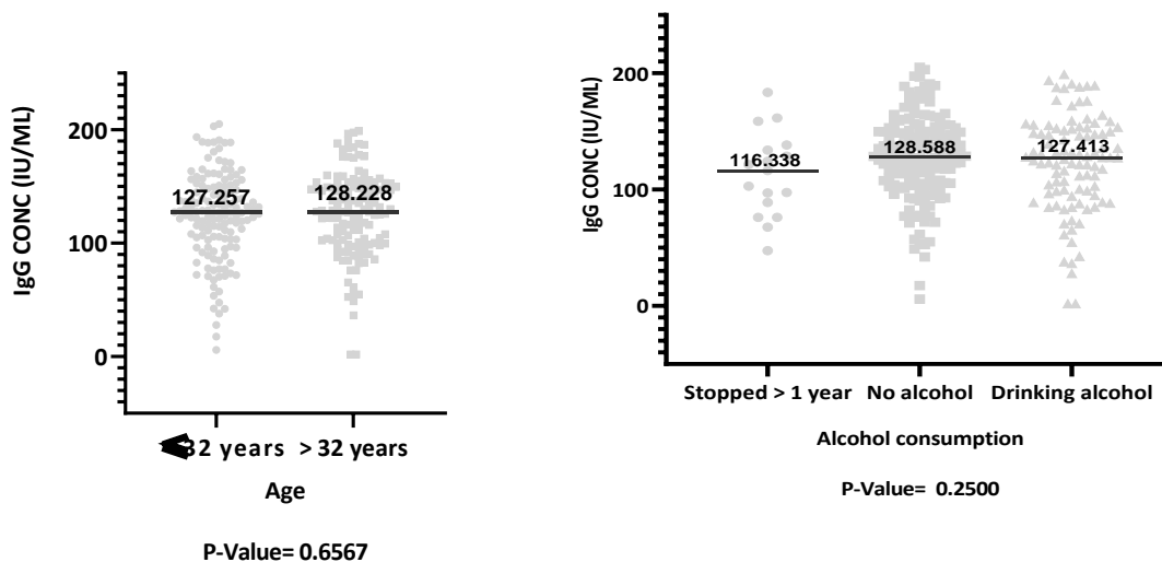
A) IgG concentration by age Category
