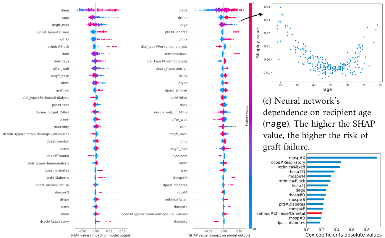
(a) Random forest SHAP-based feature importance. A positive SHAP value indicates a positive impact on graft failure.
